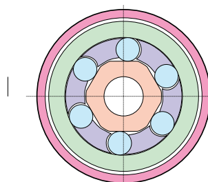
Overrunning clutch for two directions of rotation, automatic change of direction
